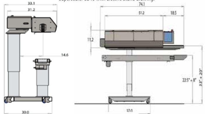
Supersealer SB40 with Electric Stand drawing.
