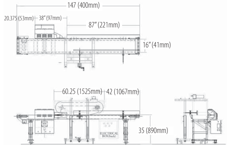
T-Pak 550 machine drawing.
