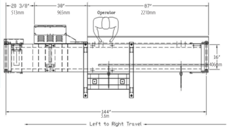
T-Pak 550 machine drawing. Drawing dimensions as reference ONLY.
