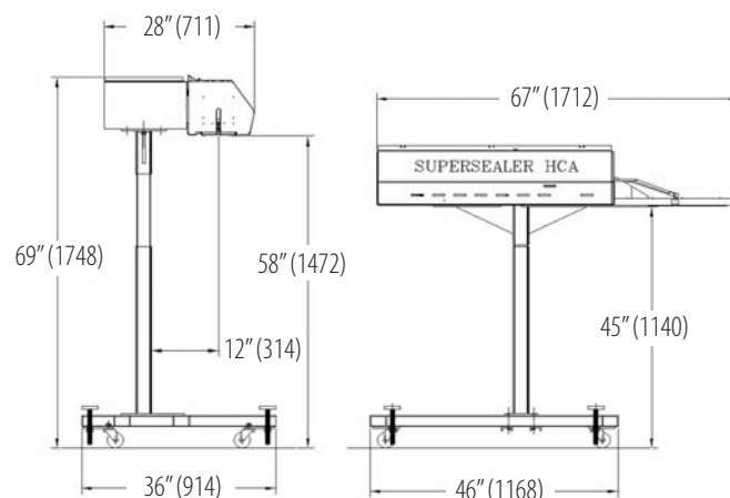
Supersealer HCA machine drawing.
